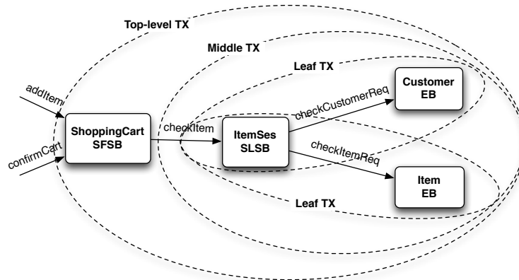
Figure 3.12: Schema of the application used as benchmark for the ONT protocol
