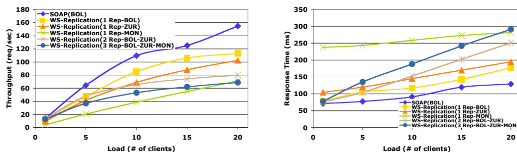
Figure 5.7: Evaluation of WS-Replication and WS-Multicast in a WAN
