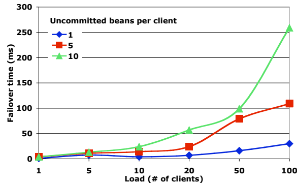
Figure 3.14: Failover time
