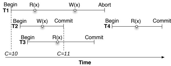
Figure 2.5: Snapshot Isolation
