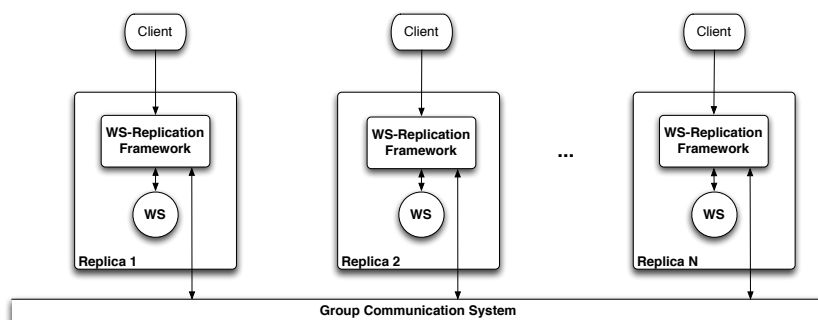
Figure 5.2: Replication model
