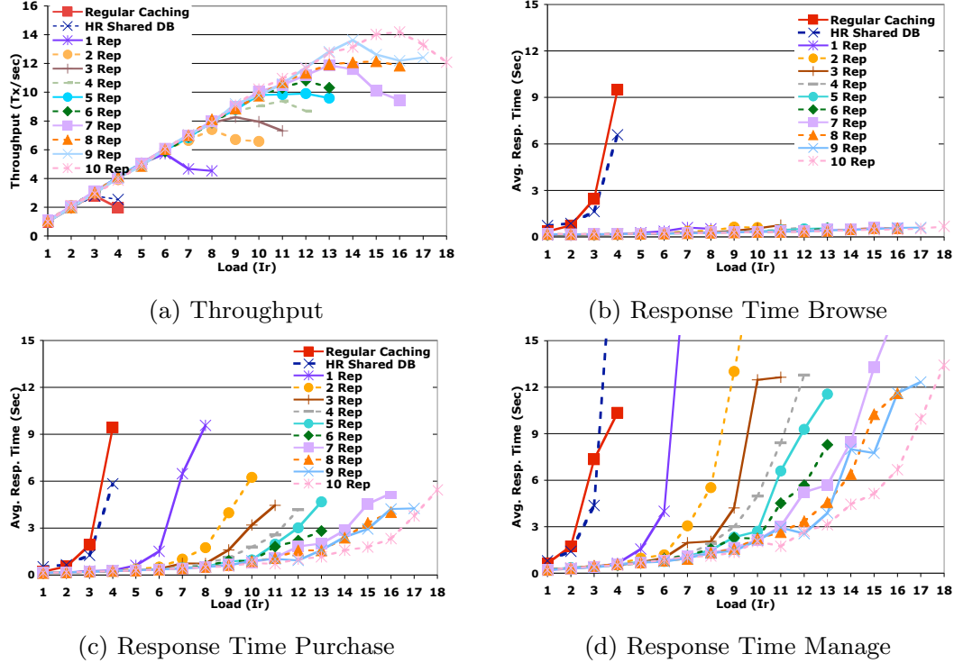
Figure 4.11: SPECjAppServer Results
