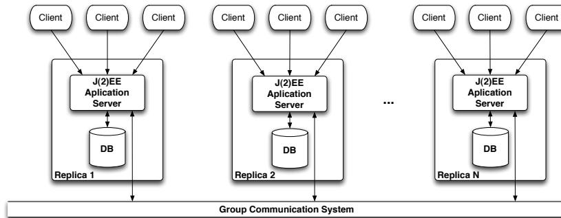
Figure 4.3: Replication model
