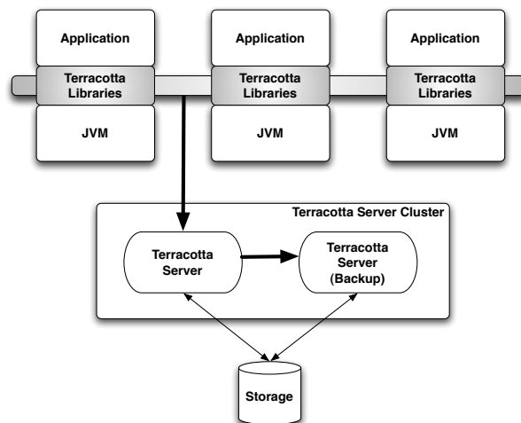
Figure 6.1: Terracotta architecture
