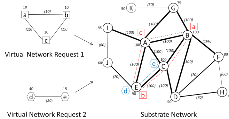
Fig. 1. An example of virtual network embedding
